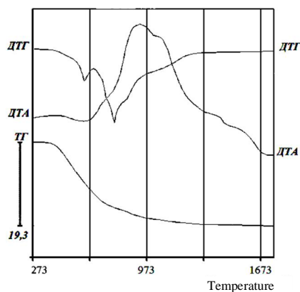
Fig. 1. Complex thermoanalysis of gap-filling \text{Al}_2\text{O}_3 , \text{ZrO}_2 and fire-clay fight of polymethylphenilsiloxane
