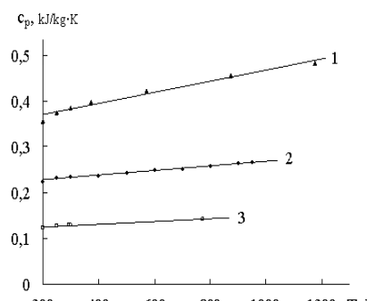
Fig. 3. Dependence of the thermal capacity ( c_p ) from temperature (T) for: 1 – copper (Z = 29), 2 – silver (Z = 47), 3 – gold (Z = 79): a - in the temperature range 0-200 K; b - in the temperature range 200-1300 K
