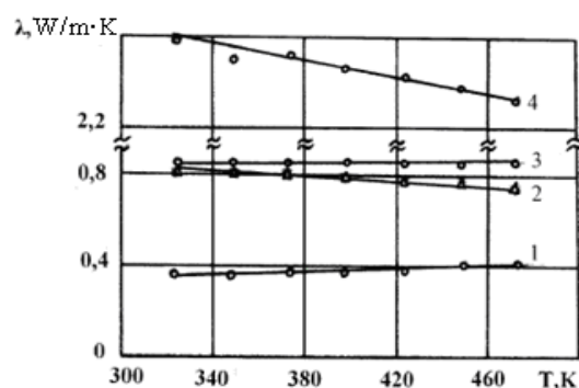
Fig. 6. The dependence of thermal conductivity ( \lambda ) from temperature (T) for composites based PTFE-4 with fillers: 1 – 25.4% vol. carbon fiber, 2 – 28 vol.% nickel powder + 2.6 vol % powdered molybdenum disulfide, 3 – 20% vol. ARV graphite powder; 4 – 28vol. % copper powder + 2.6% vol. powdered molybdenum disulfide
