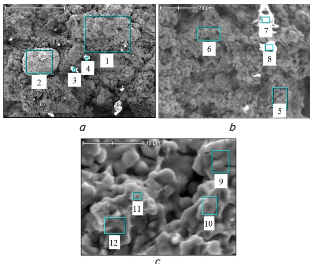
Fig. 5. Images of the microstructure of metallized molybdenum concentrate at magnification: a – ×50, b – ×1000, c – ×5000
