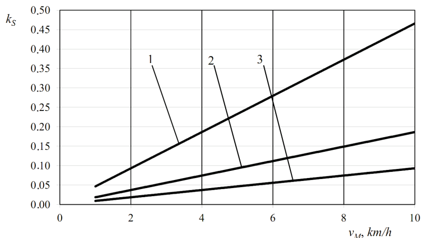
Fig. 4. Calculation and experimental dependences of the grain separation coefficient ( k_s ) on the combine harvester speed ( v_M ) under conditions m_c=3.5 kg; q=8 kg/s; \beta=1.3 , for different l_i : 1 – l_i=6 m; 2 – l_i=15 m; 3 – l_i=30 m
