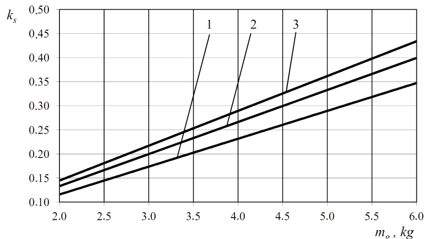
Fig. 5. Calculation and experimental dependences of the separation coefficient of grain ( k_s ) on the mass of the grain separated by the device by l_i=6 m; v_M=5 km/h; q=8 kg/s for various \beta : 1 – \beta=1.0 ; 2 – \beta=1.3 ; 3 – \beta=1.5
