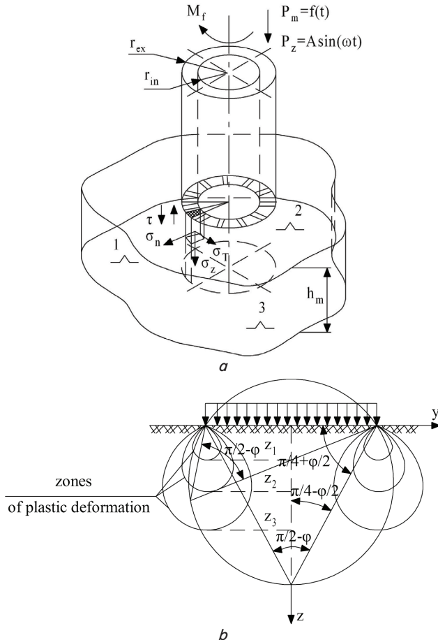
Fig. 2. Tubular drill:
