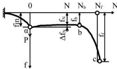
Fig. 2. Curve of sample deflection measurement [8]: N f – number of cycles to sample failure; f in – initial deflection value; f f – deflection in the moment of failure; f N – current deflection; \Delta f_N – alteration of current deflection; b – point that corresponds to the moment of fatigue crack initiation; ( ab ) – section of the deflection curve before crack initiation; ( b-c ) – section of crack propagation; f b – deflection in the moment of fatigue crack initiation
