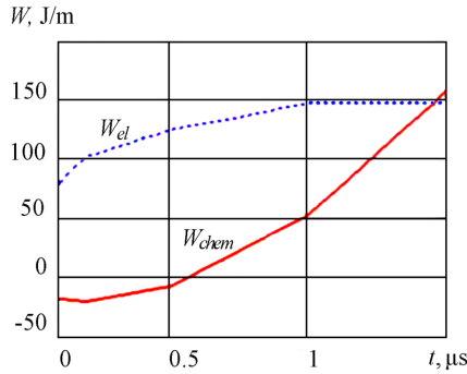
Fig. 3. Change in the amount of electric energy W_{el} ----- and energy W_{chem} , released (absorbed) during chemical reactions ———
