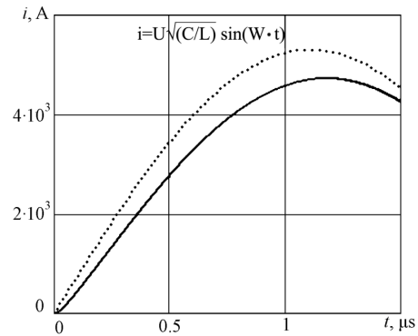
Fig. 1. Specified current curve
