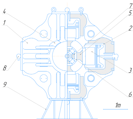
Fig. 1. General view of the pressing unit CS-VII [6]:
