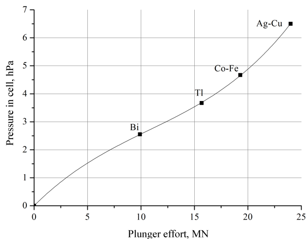
Fig. 12. Load characteristic of the pressing unit CS-VII when using the fixed points of phase transitions in bismuth and thallium at room temperature and differential temperature differences \text{Co}^{\alpha-\beta} - \text{Fe}^{\alpha-\gamma} and \text{Ag}^I - \text{Cu}^I (Fig. 5) when T = 563.9 – 642.7 °C – p = 4.67 hPa and at T = 1,305.7 – 1,313.5 °C – p = 6.5 hPa, respectively
