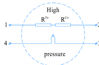
Fig. 7. A principal electric diagram of connecting the wires of iron and cobalt for the sensor Co–Fe: 1, 2 – connection of the sensor Co–Fe to punches 1 and 2 of the pressing unit; 3, 4 – connection of the thermocouple sensor to punches 3 and 4 of the pressing unit
