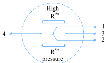
Fig. 9. A principal electric diagram of connecting the wires of copper and silver for the melting sensor: 1, 2 – connection of the thermocouple sensor to punches 1 and 2 in the pressing unit; 3, 4 – connecting the melting sensor Ag–Cu to punches 3 and 4 in the pressing unit
