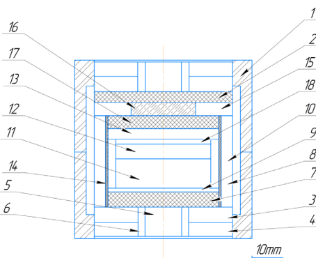
Fig. 2. Schematic of a high-pressure cell in a cubic container of the six-punch HPU CS-VII for determining values for transformations in sensors Co–Fe or Ag–Cu: 1 – semi-cubes 58x58x29 mm a dolomitic insert and an axial hole of Ø44 mm; 2 – graphite current distributing disk; 3 – heat insulating dolomitic ring; 4 – heat insulating pyrophyllite ring; 5 – heat insulating dolomitic disk; 6 – steel current connection; 7, 17 – graphite current distributing disk; 8 – heat insulating bushing made of CsCl; 9, 13 – discs made of CsCl; 10 – ring made of CsCl; 11 – alloy, a carbon solvent; 12 – source of carbon, graphite; 14 – cylinder graphite heater; 15 – heat insulating ring made of CsCl–ZrO 2 ; 16 – heating element from a mixture of graphite and ZrO 2 ; 18 – sensor placement in a cell
