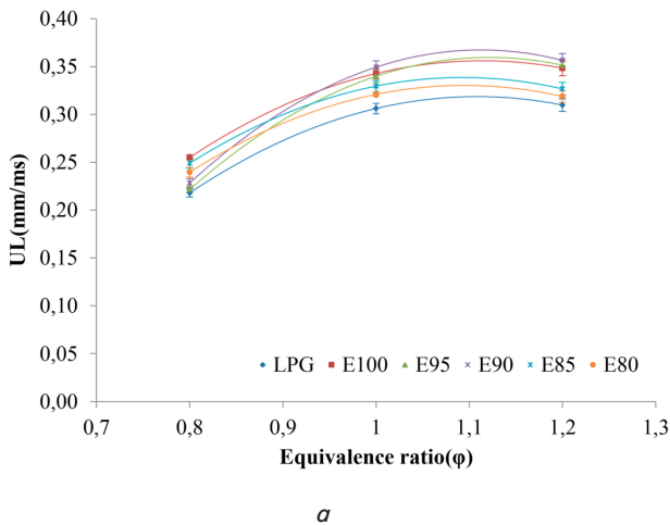
Fig. 6. Laminar burning velocity ( U_L ): a – various fuel compositions; b – Hydrus E90
