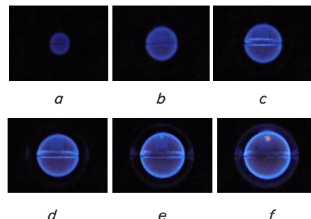
Fig. 2. Flame propagation in a stoichiometric mixture of E90, time interval 2.3 ms: a – 2.3 ms; b – 4.6 ms; c – 6.9 ms; d – 9.1 ms; e – 11.4 ms; f – 13.7 ms
