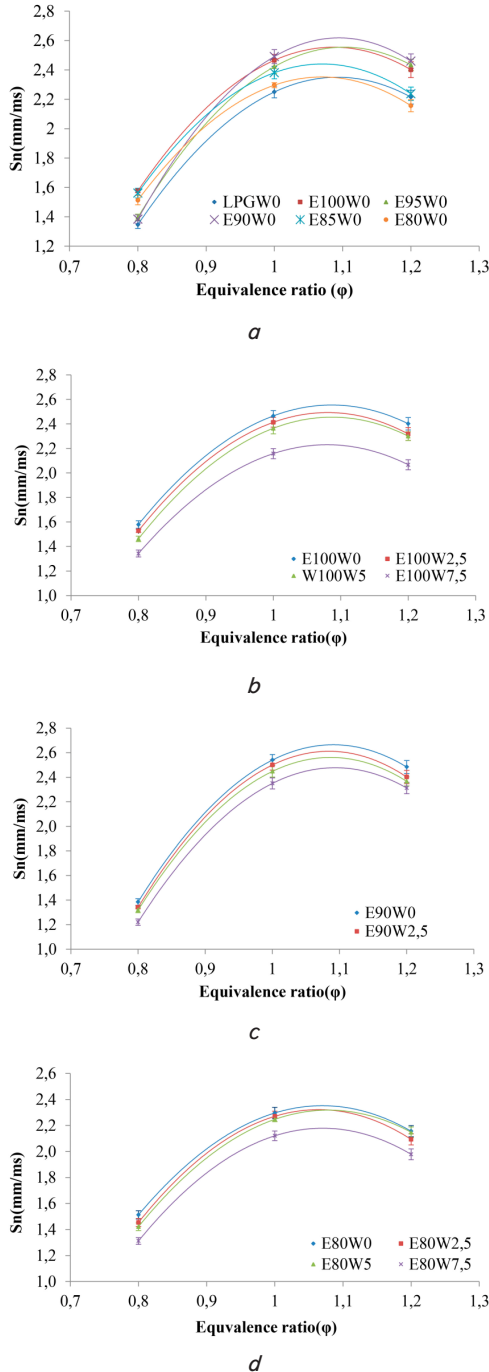
Fig. 3. Stretched flame speed ( S_n ) of various fuel compositions versus equivalence ratio: a – pure fuels and anhydrous composition; b – hydrous ethanol; c – hydrous E90; d – hydrous E80
