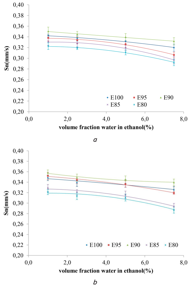
Fig. 7. Laminar burning velocity for ethanol with LPG addition as a function of volume fraction of water in ethanol: a – \phi=1.0 ; b – \phi=1.2
