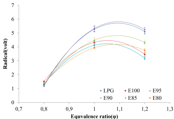
Fig. 9. Relationship between the radicals concentration against equivalence ratio
