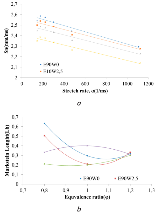
Fig. 4. Dependence of stretch and equivalence ratio on the flame speed and Markstein length of hydrous E90: a – Stretched flame speed; b – Markstein length
