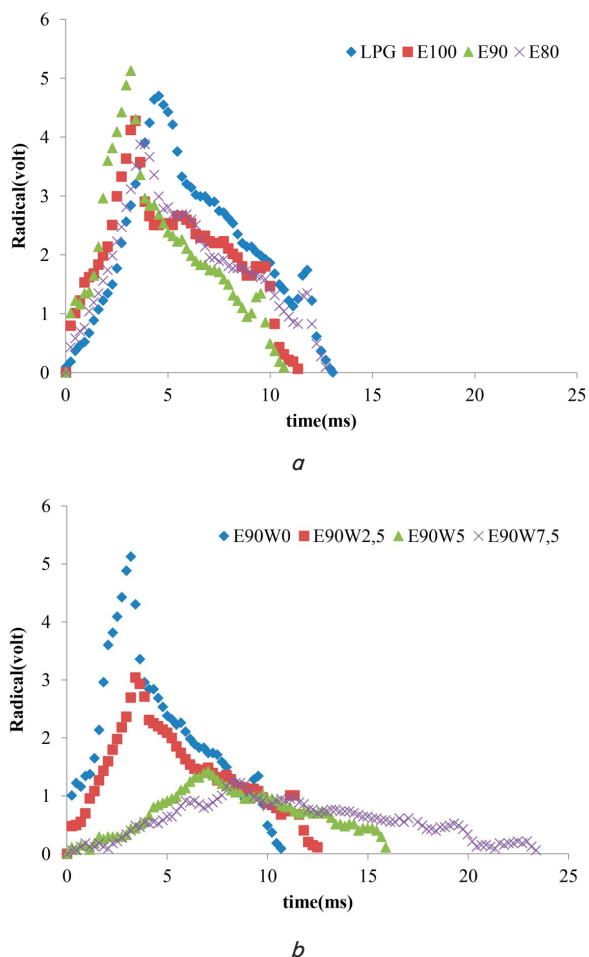
Fig. 8. Measured voltage (radical) against the combustion time at \phi=1 : a – anhydrous composition; b – hydrous E90
