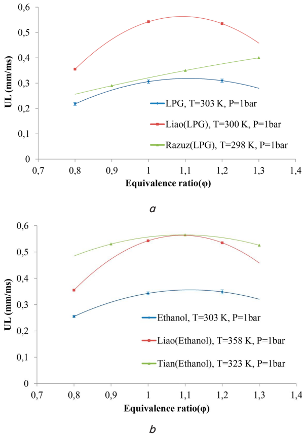
Fig. 5. Laminar burning velocity ( U_L ) of pure fuel: a – LPG; b – Ethanol
