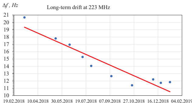
Fig. 4. Long-term drift of assigned value for 223 MHz frequency
