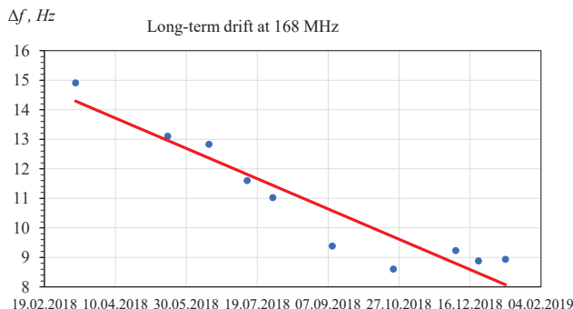
Fig. 3. Long-term drift of assigned value for 168 MHz frequency
