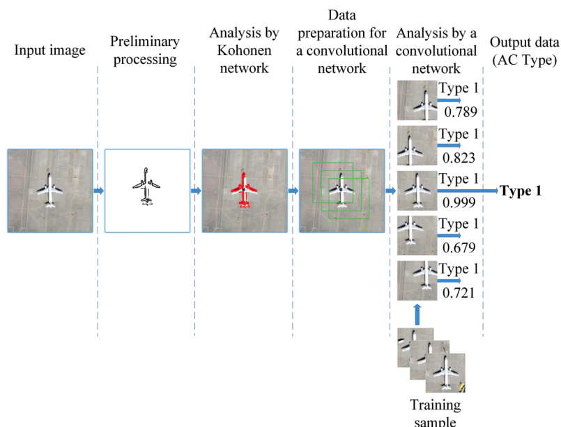
Fig. 2. Operation scheme of the algorithm for searching the ROIs and determination of a type of AC
