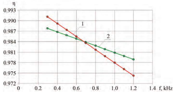
Fig. 7. Dependence of efficiency on switching frequency: 1 – two-level active rectifier; 2 – three-level active rectifier
