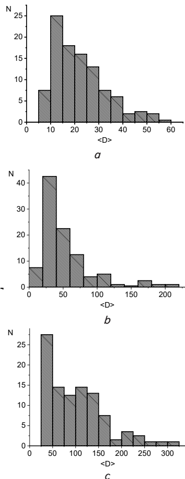
Fig. 3. The distribution, based on size of mean diameters ( \langle D \rangle , \mu\text{m} ), of grains of former austenite in steel 40X after hardening at temperatures: a – 860 ^{\circ}\text{C} ; b – 950 ^{\circ}\text{C} ; c – 1,050 ^{\circ}\text{C} (exposure to hardening – 30 min)
