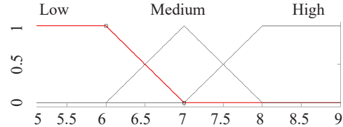
Fig. 8. Input variable (Weld current) membership function
