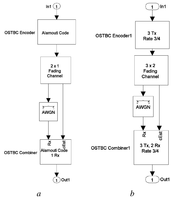
Fig. 1. MIMO 2×1 Channel ( a ), MIMO 3×2 Channel ( b )
