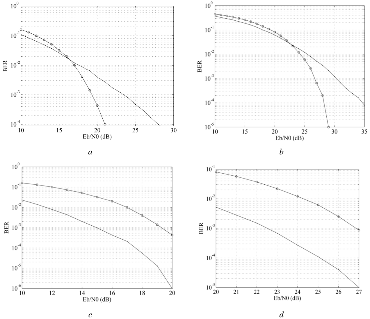
Fig. 3. Dependence of an error probability for a BPSK (a, c) and a QPSK (b, d) modulation scheme on a ratio E_b/N_0 in uplink/downlink channels: a, b: dots – MIMO 2×1 uplink/downlink channels, circles – AWGN uplink/downlink channels; c, d: dots – MIMO 3×2 uplink/downlink channels, circles – AWGN uplink/downlink channels
