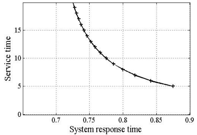
Fig. 5. System response time with fixed rate of arrival
