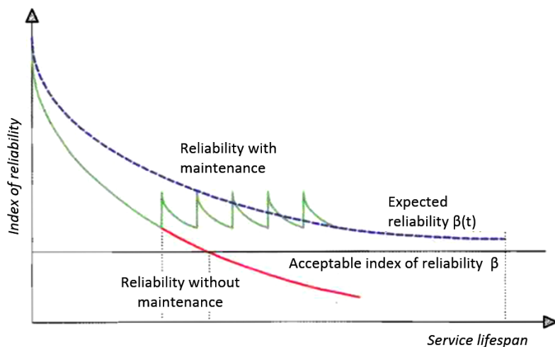
Fig. 4. Possibilities of reliability change in construction lifespan due to structure maintenance
