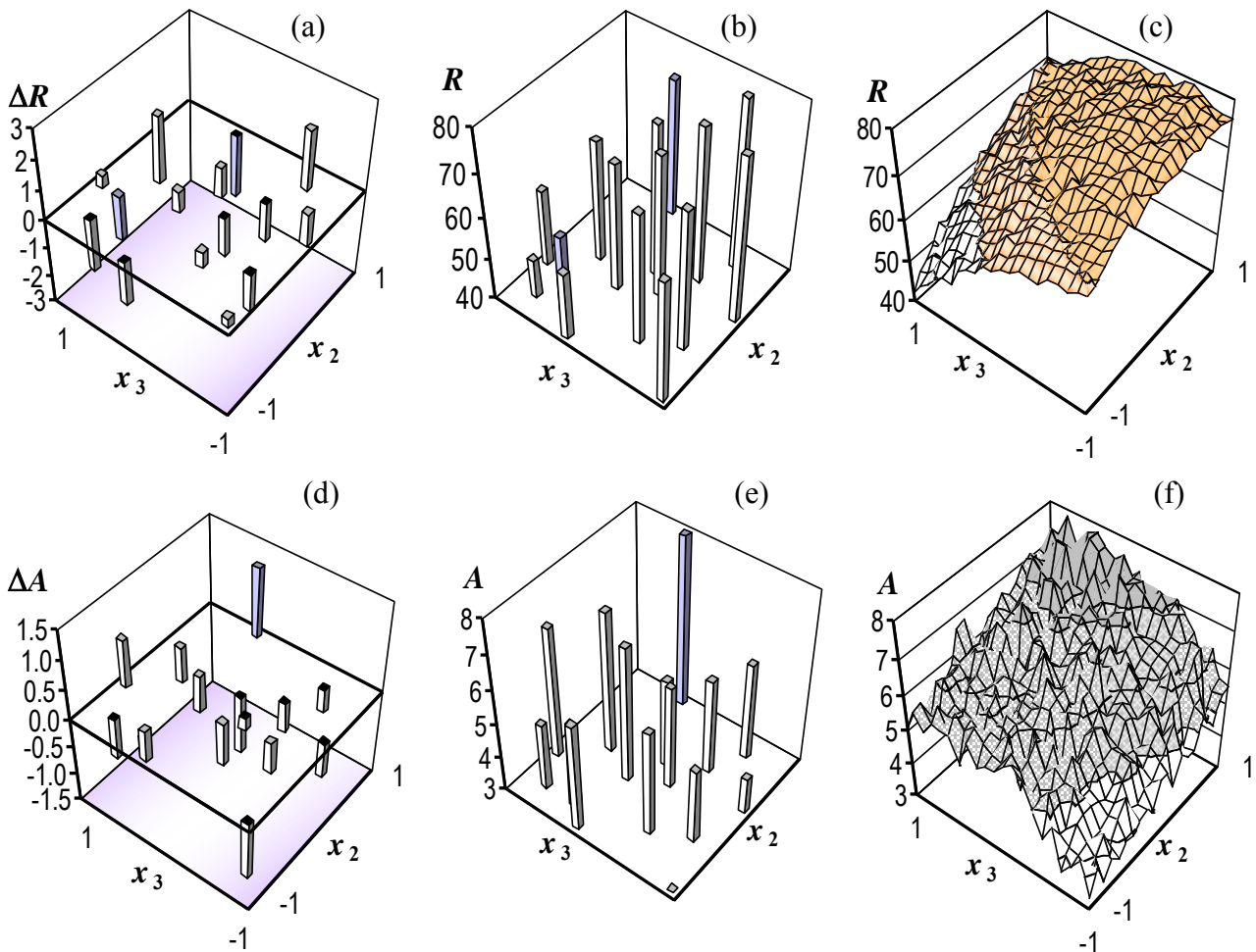
Fig. 3. Generated random errors and property levels for a number of generated compositions and one realisation of random field for compression strength (a-c) and abrasion resistance (d-f)
