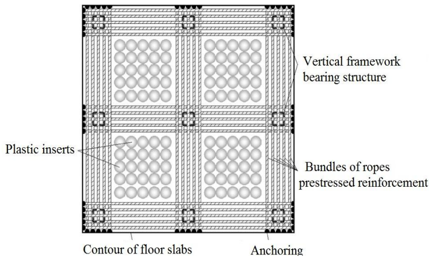
Fig. 3. The structure of monolithic prestressed slab with non-removable inserts
