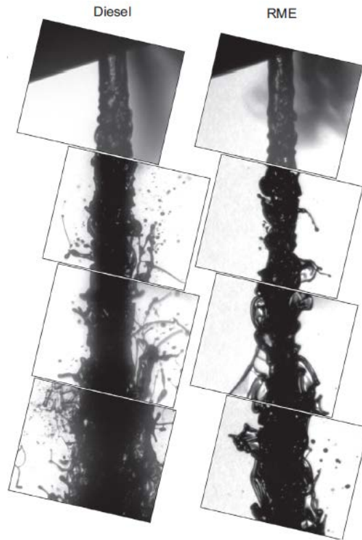
Figure 1. Influence of fuel type on the primary atomisation within the first 2.1 mm from the nozzle (left is diesel fuel and right is biodiesel (RME)). Injection pressure is 40 MPa; gas pressure is 0.1 MPa [12]
