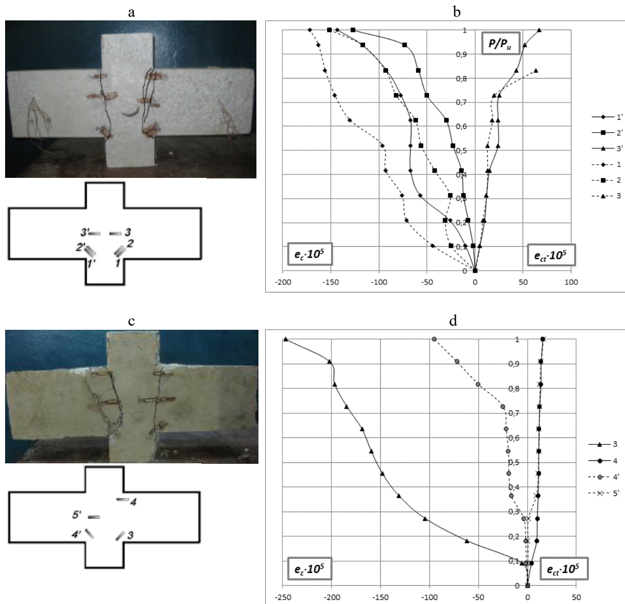
Figure 6 – The failure character (a) and diagram « \varepsilon_c (\varepsilon_{ct}) - P/P_u » (b) for reinforced concrete keys with one-level and two-level (c, d) plating of reinforcement
