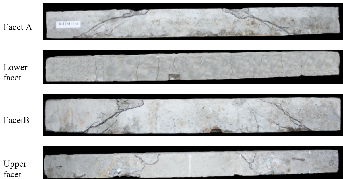
Figure 10 – Failure character of testing beam B-HS-1-a
