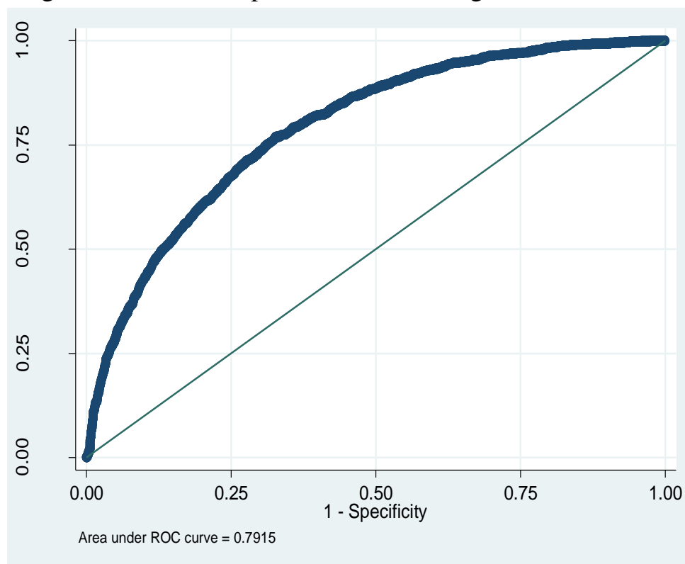
Fig. 1. ROC curve
