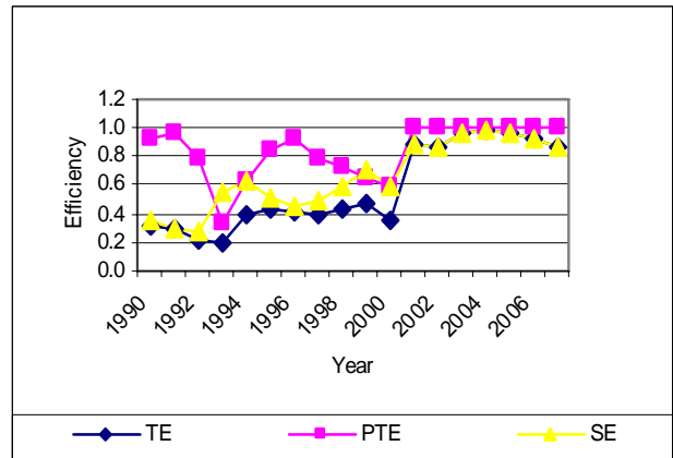
Fig. 13. Technical, pure technical and scale Efficiencies – state banks
