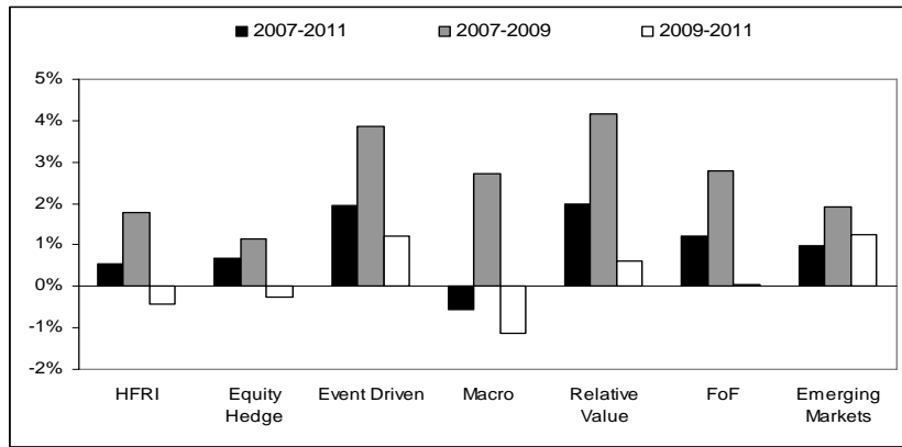
Fig. 4. Monthly \alpha_{leverage} for the different HFR indices
