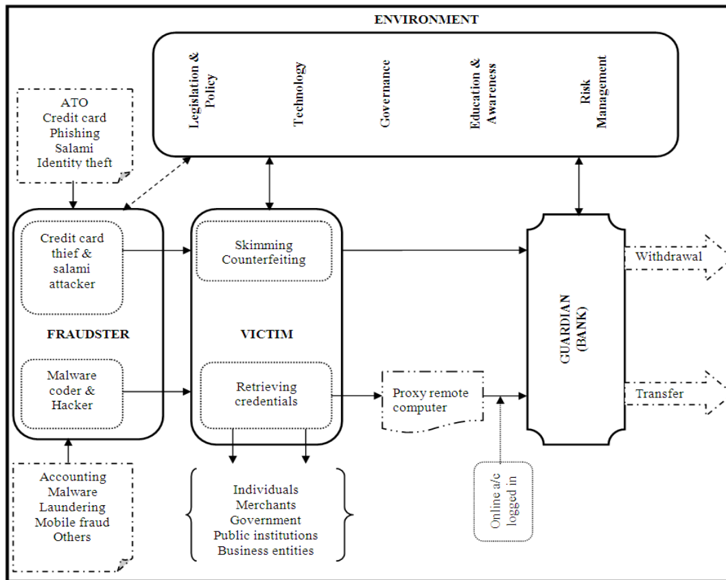
Fig. 4. Proposed framework
