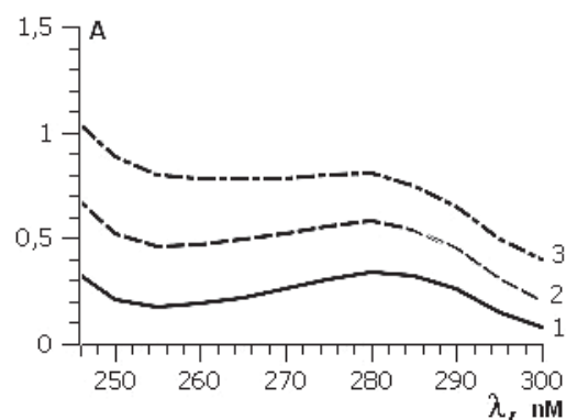
Fig. 2. The absorption spectra of BSA solutions in the UV wavelength range, comprising: A_{\text{BSA}} - solid line, BSA; A_{0.1\text{Cu}} - dotted line, BSA + 20 mM NaCl + 0.1 mM \text{CuCl}_2 ; A_{0.4\text{Cu}} - dash-dotted line
