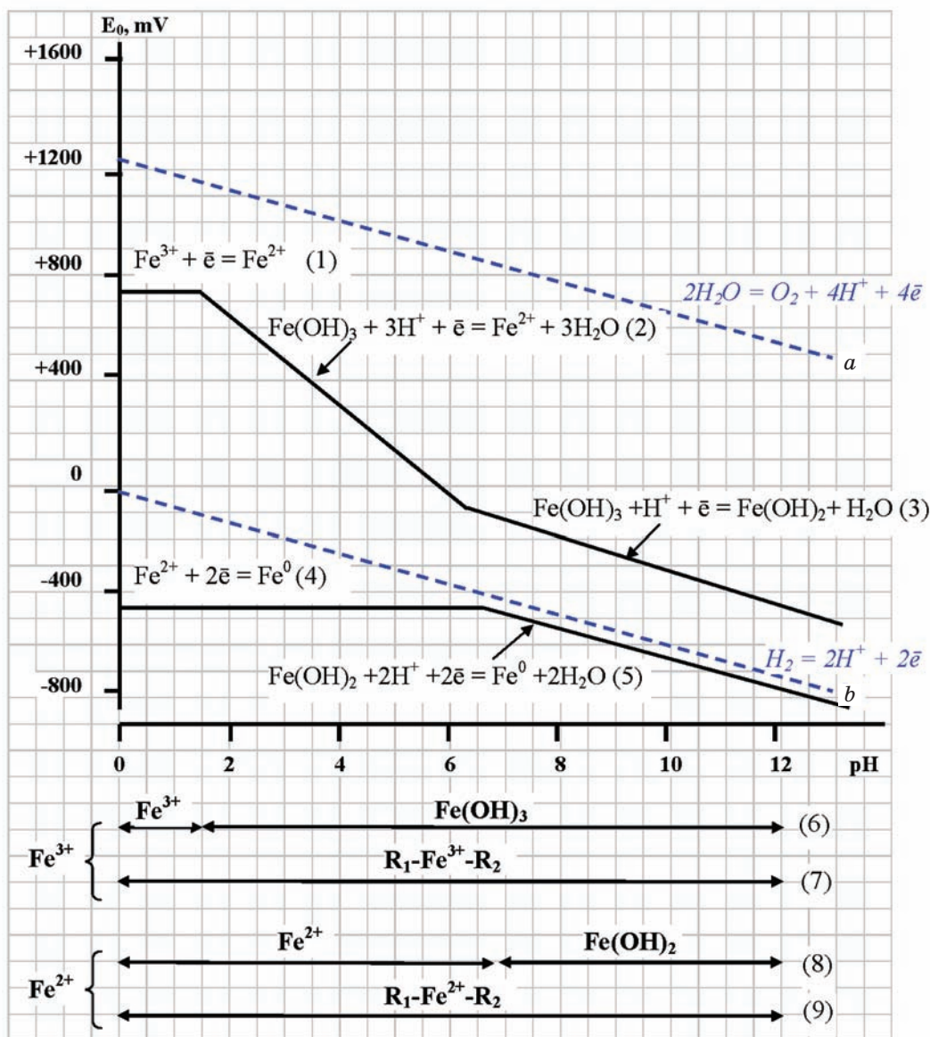
Fig. 1. Zones of redox-stability of Fe(II) and Fe(III) compounds: a (top) and b (lower) — limit of thermodynamic stability of water: a — is described by the equation: \text{O}_2 + 4\text{H}^+ = 2\text{H}_2\text{O} and E_h = 1.228 - 0.0591 \cdot \text{pH} - 0.0295 \cdot \lg \text{PH}_2 ; b — is described by the equation: 2\text{H}^+ + 2e = \text{H}_2 and E_h = 0.000 - 0.0591 \cdot \text{pH} - 0.0591 \cdot \lg \text{PH}_2 ; \text{R}_1^- , \text{R}_2^- — organic radicals (organic acids or amino acids)
