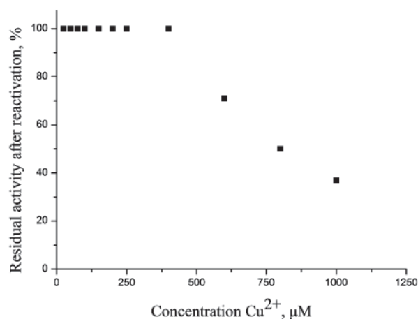
Fig. 5. Dependence of biosensor reactivation level after inhibition by Cu 2+ ions with different concentrations.
