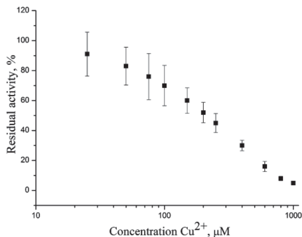
Fig. 3. Residual activity of urease biosensor after inhibition by Cu 2+ ions with different concentrations. Inhibition time — 20 minutes.
