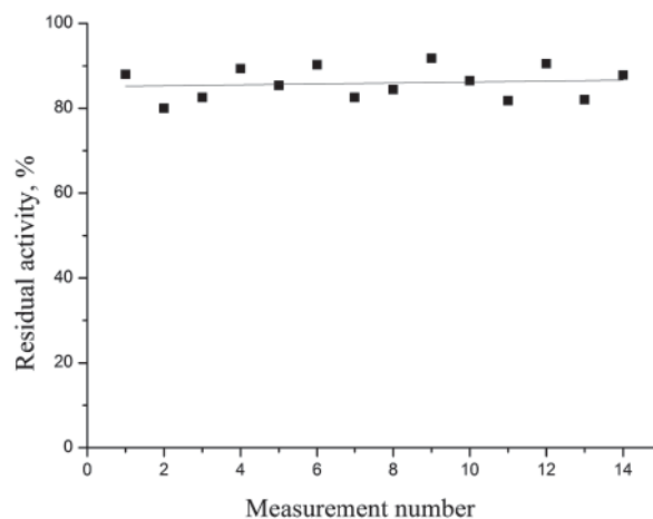
Fig. 4. Reproducibility of urease biosensor after inhibitory analysis. Inhibitor concentration — 50 µM Cu 2+ . Inhibition time — 20 minutes.
