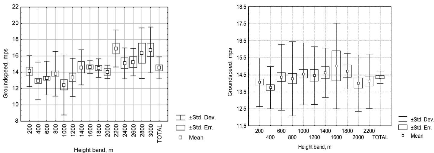
Fig. 2. The box plots of bird groundspeeds per altitude bands in spring (left) and autumn (right), 2001.
