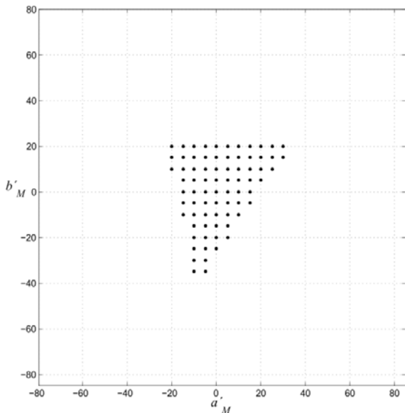
Figure 9 – Color points of color gamut transmitted and reproduced by HDTV system for J' = 30 on the a'_M, b'_M plane of the CAM02–UCS space
