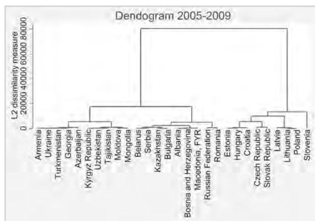
Fig. 2: Dendrogram of clusters for the 2005-2009 period Source: Authors' calculations
