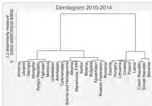
Fig. 3: Dendrogram of clusters for the 2010-2014 period Source: Authors' calculations
