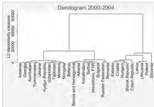
Fig. 1: Dendrogram of clusters for the 2000-2004 period Source: Authors' calculations
