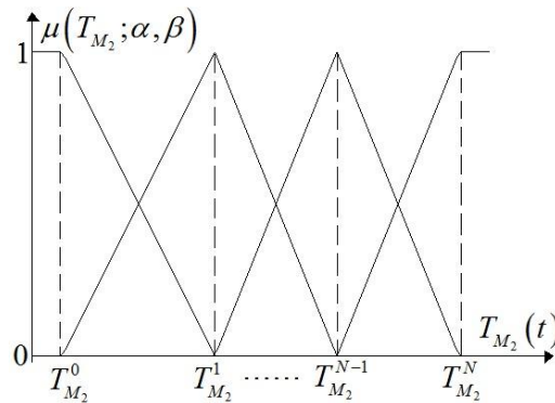
Fig. 2. Membership function
