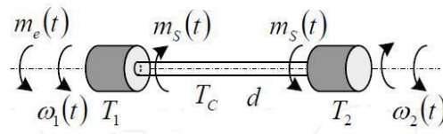
Fig. 1. Typical scheme of a two-mass system
