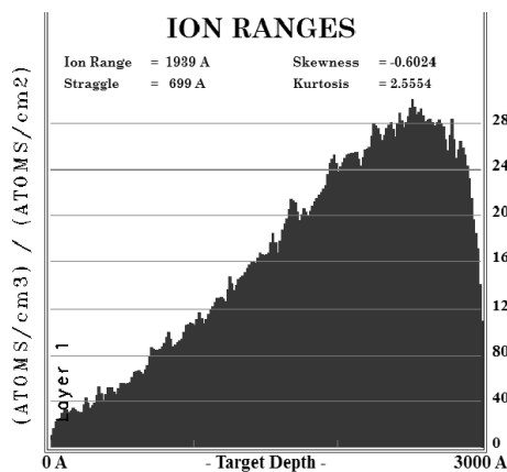
Fig. 6. Distribution of iron ions in the zirconium-iron alloy layer with a layer depth of 300 nm
