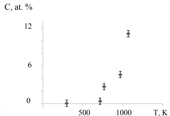
Fig. 3. Dependence of iron concentrations in the surface layer Depth 300 nm of the alloy from the thermal annealing temperature of the deformed layer Zr-1.03 at.% Fe
