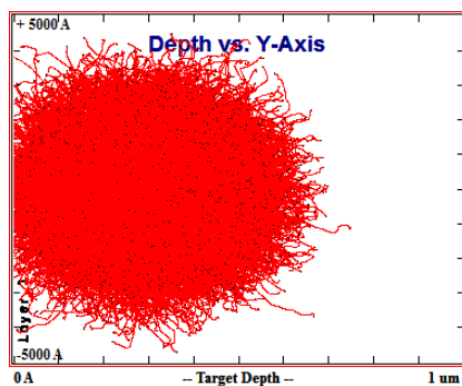
Fig. 4. Damage cascade with energy of 600 keV ions
