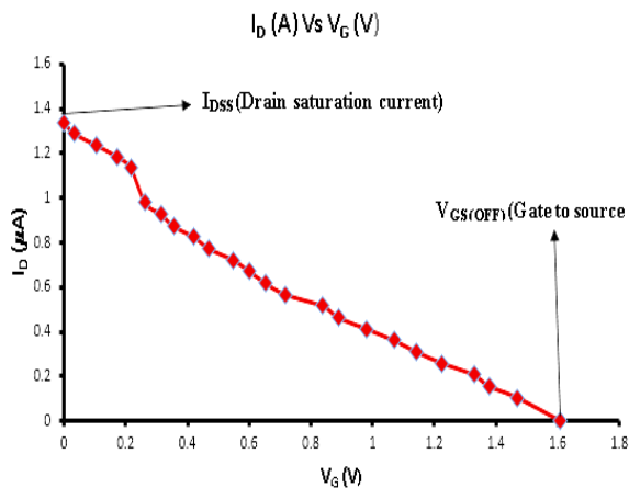
Fig. 9. Transfer curve of SnS honey gated EDLFET
