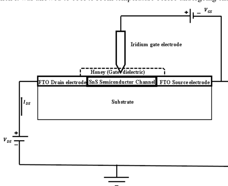
Fig. 1. A schematic diagram of the SnS EDLFET
