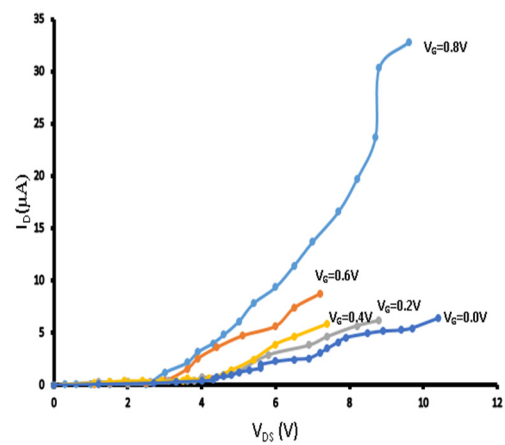
Fig. 10. Output curve of SnS honey gated EDLFET
