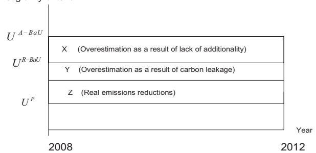
Fig. 1. Illustration of the different sources for overestimation of annual emissions reductions from CDM-projects
