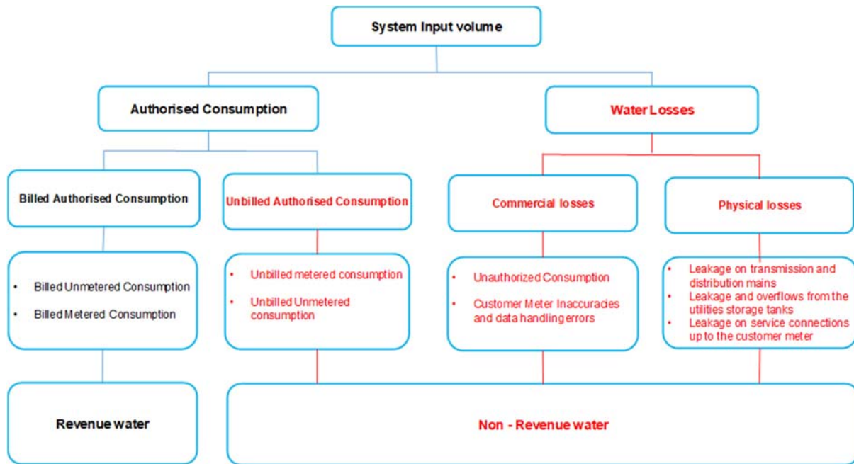
Fig. 2. The IWA best practice standard water balance
