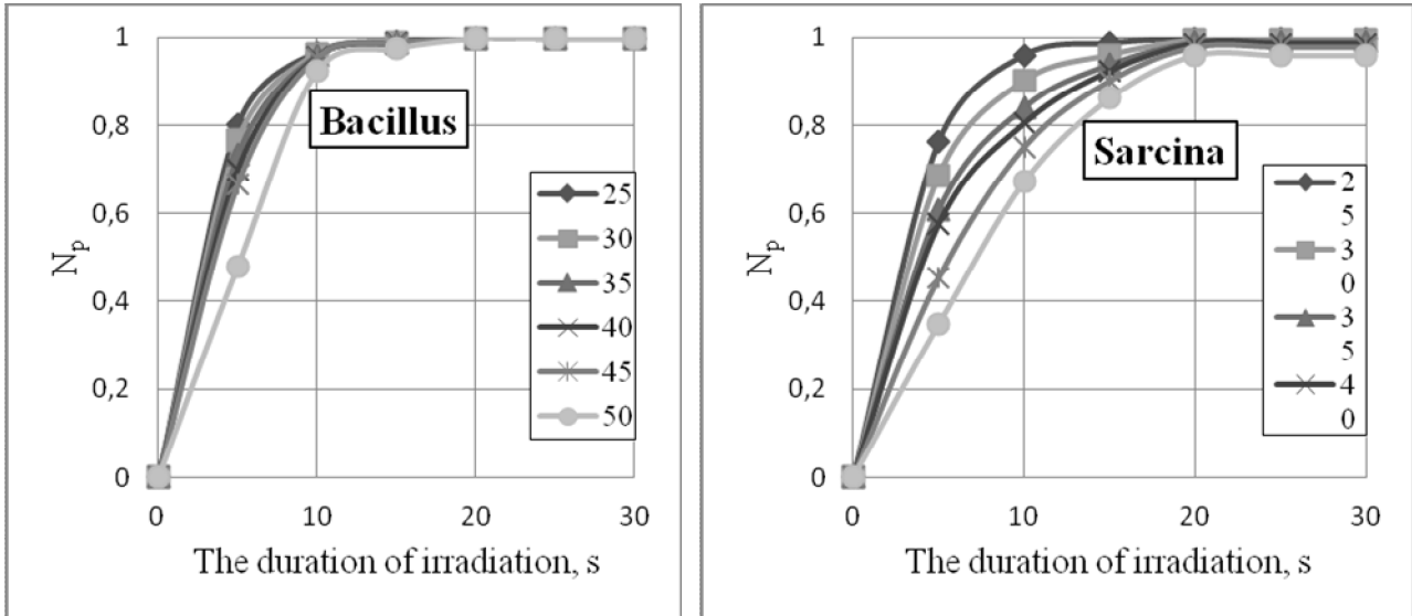
Fig. 3. Kinetics of changes in the degree of purification during the process of UV irradiation against different types of bacteria and for different layer thickness of polluted water (mm)
