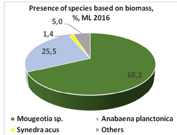
Fig. 4. Percentage ratio of phytoplanktonic divisions and species based on the biomass (%) in ML in 2016
