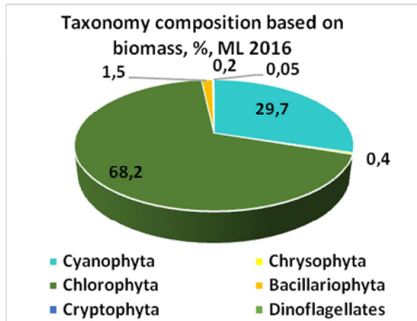
Fig. 4. Percentage ratio of phytoplanktonic divisions and species based on the biomass (%) in ML in 2016
