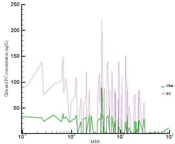
Fig. 6. Chlorophyll-a and Phycocyanin versus MRR (field data 2015 and 2016)
