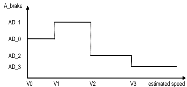
Fig. 5. The braking force A_{brake} vs. estimated speed V
