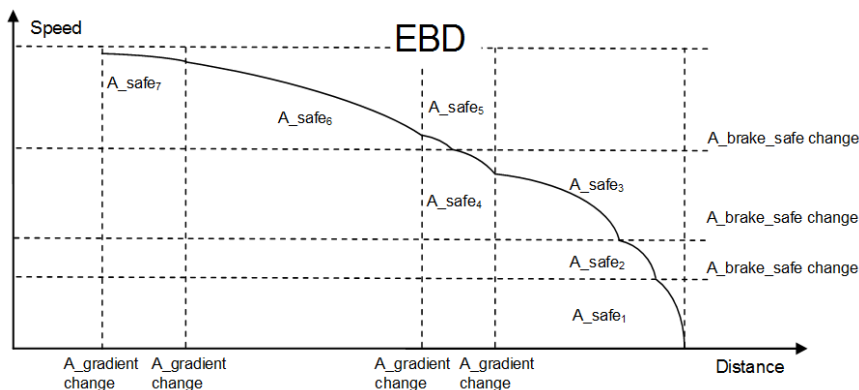
Fig. 6. Construction of the EBD [15]
