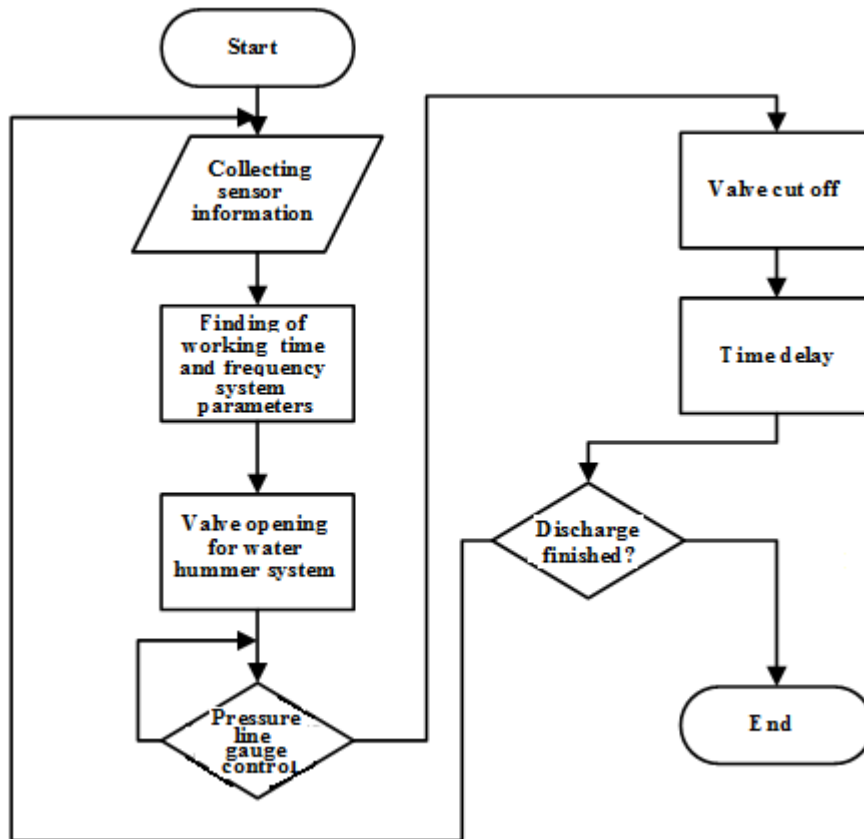
Fig. 3. Scheme of the algorithm for valve control
