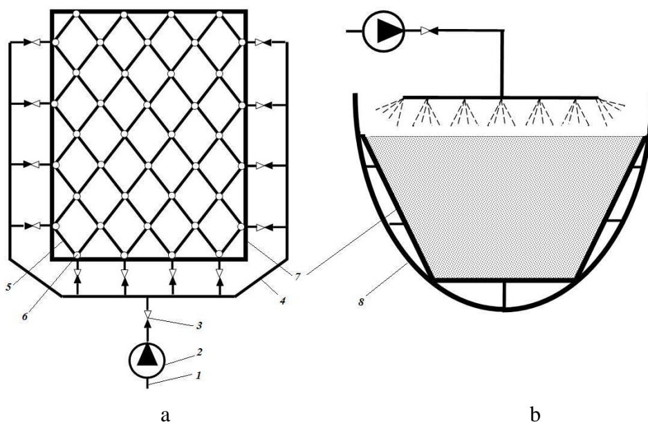
Fig. 1. Scheme of washout system a – top view, b – lateral view: 1 – feed pipeline; 2 – pump; 3 – electromagnetic valve; 4 – loop pipeline circuit; 5 – washout pipeline; 6 – washout hole; 7 – vessel's tank; 8 – vessel's hull
