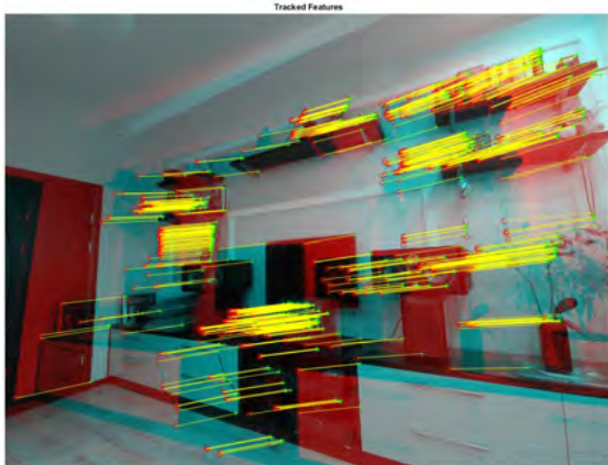
Fig. 11 Tracked features
