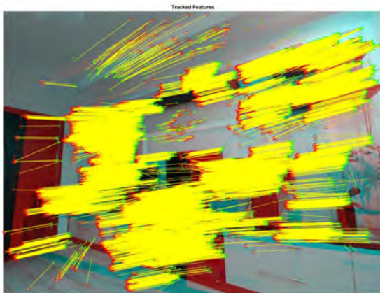
Fig. 5. Matched features
