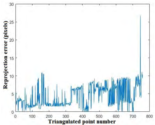
Fig. 13. Reprojection error graph
