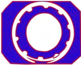
Fig. 7. Cut of plasma with a localized discharge on condition, that 650.37 \leq p \leq 1090.6 Pa
