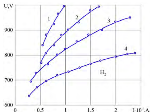
Fig. 3. Volt-ampere characteristics of a localized discharge, on condition of hydrogen pressure changing: 1 – p = 18.62 Pa ; 2 – p = 25.27 Pa ; 3 – p = 39.91 Pa ; 4 – p = 53.27 Pa
