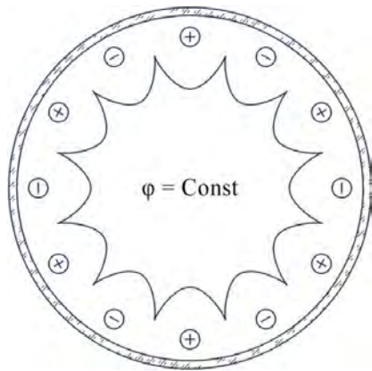
Fig. 1. Electrostatic field of a localized discharge interval: + anodes; – cathodes
