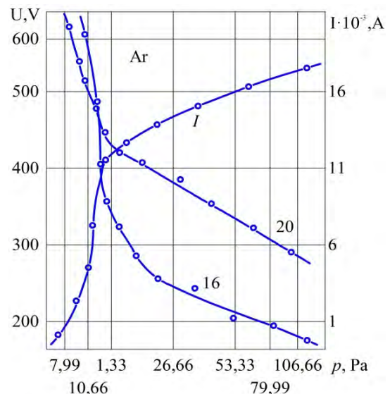
Fig. 5. Dependence of arcing tension U and current I in the localized discharge, from argon pressure, when U = \varphi(p) , if I = \text{const} ; I = f(p) , if U = \text{const} , likewise 16 - U = \varphi(p) in case of 16 electrodes and 20 - U = \varphi(p) in case of 20 electrodes
