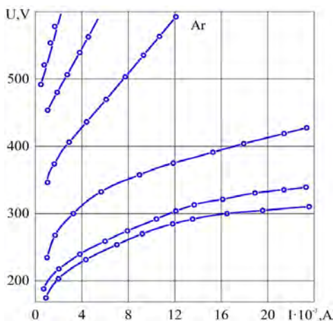
Fig. 2. Volt-ampere characteristics of a localized discharge, on condition of argon pressure changing: 1 – p = 2.66 Pa ; 2 – p = 5.32 Pa ; 3 – p = 7.98 Pa ; 4 – p = 13.3 Pa ; 5 – p = 53.2 Pa ; 6 – p = 79.8 Pa
