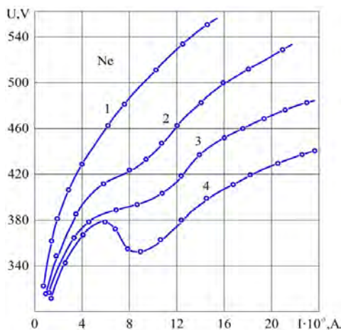
Fig. 10. Discharge volt-ampere characteristics, on condition of rod electrodes different lengths, when neon pressure p = 17.29 Pa : 1 – l_1 = 0.13 m ; 2 – l_2 = 0.14 m ; 3 – l_3 = 0.15 m ; 4 – l_4 = 0.16 m
