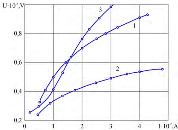
Fig. 8. Volt-ampere characteristics of a localized discharge according to the different pressures in neon: 1 – p_1 = 650.37 Pa ; 2 – p_2 = 824.6 Pa ; 3 – p_3 = 1103.9 Pa
