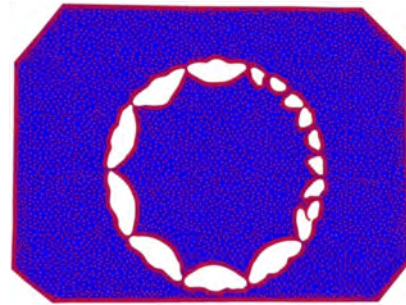
Fig. 9. Radiation of plasma's column, when p > 1090.6 Pa
