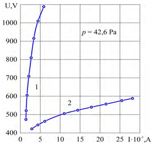
Fig. 4. Comparison of volt-ampere characteristics of a localized discharge – 2 and discharge that glows with flatly-parallel interval – 1, on condition of identical cathode area, energy contribution and pressure
