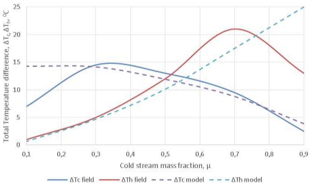
Fig. 7. Comparison of simulation results and experimental data at P_i = 2 \text{ atm} , T_i = 30 \text{ }^\circ\text{C}
