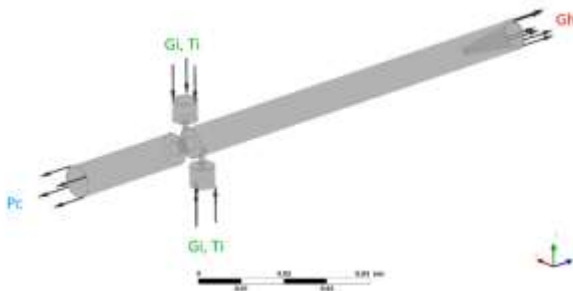
Fig. 4. Boundary conditions
