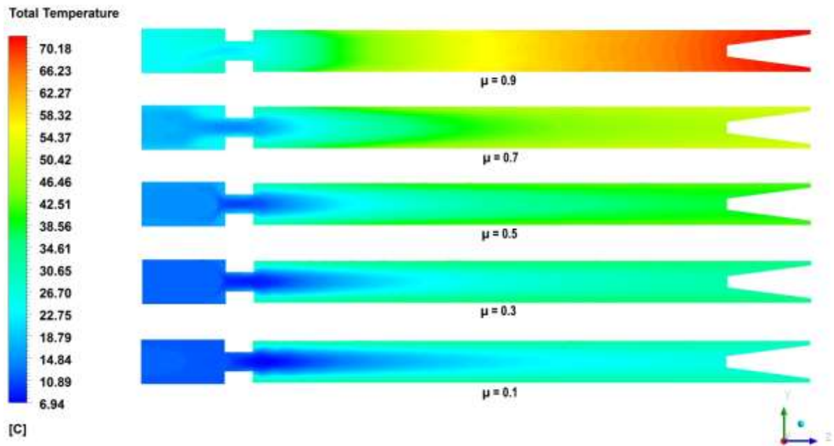
Fig. 6. Contours of total temperature in YZ plane
