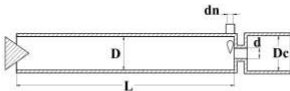
Fig. 1. Schematic view of the vortex tube geometry
