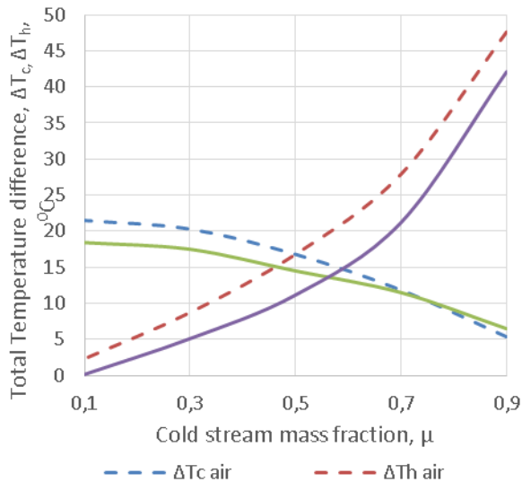
Fig. 11. The total temperature differences for air and methane, P_i \approx 4 atm
