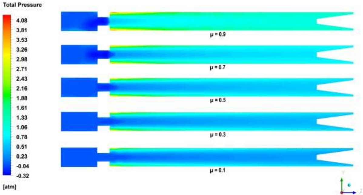
Fig. 5. Contours of total pressure in YZ plane
