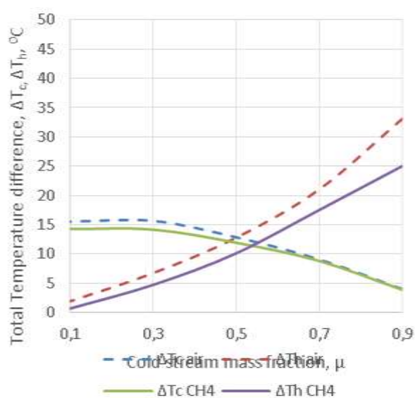
Fig. 9. The total temperature differences for air and methane, P_i \approx 2 \text{ atm}
