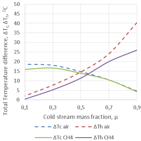
Fig. 10. The total temperature differences for air and methane, P_i \approx 3 atm
