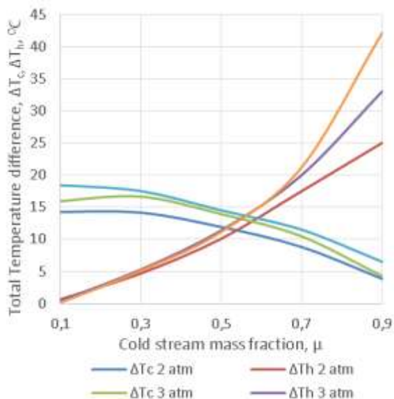
Fig. 8. The total temperature differences at different levels of inlet pressure
