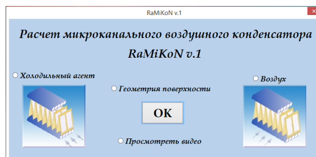
Figure 2 – Main window
