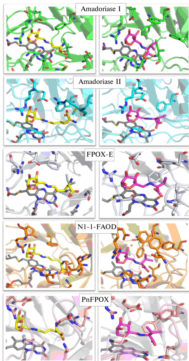
Fig. 6. Ligand binding residues. The residues forming relevant interactions (polar or hydrophobic) with f-lys (yellow) and f-val (pink) within the catalytic pocket are shown for each enzyme
