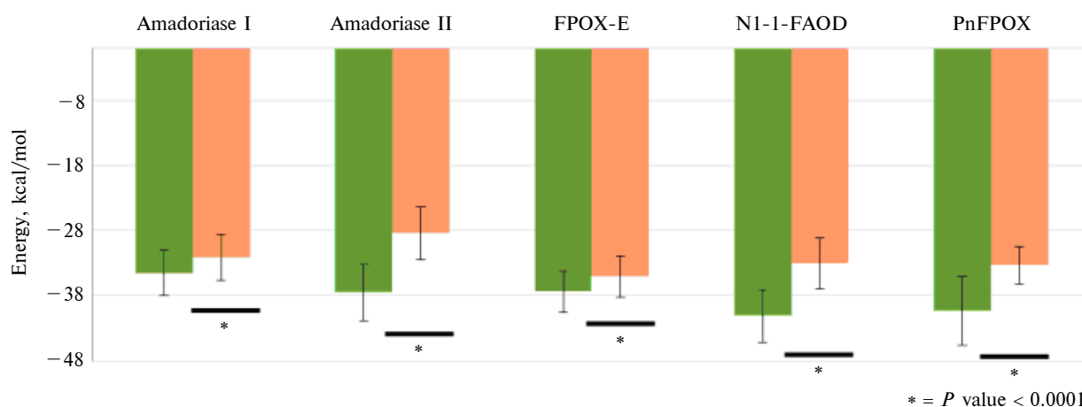
Fig. 7. MM-PBSA calculations. For each enzyme, the values of the enthalpic component of the binding free energy are reported for the two different ligands. All enzymes show similar binding energies when in complex with the same ligand. Moreover, they all show a lower binding energy for f-lys compared to f-val: ■ – f-lys; ■ – f-val
