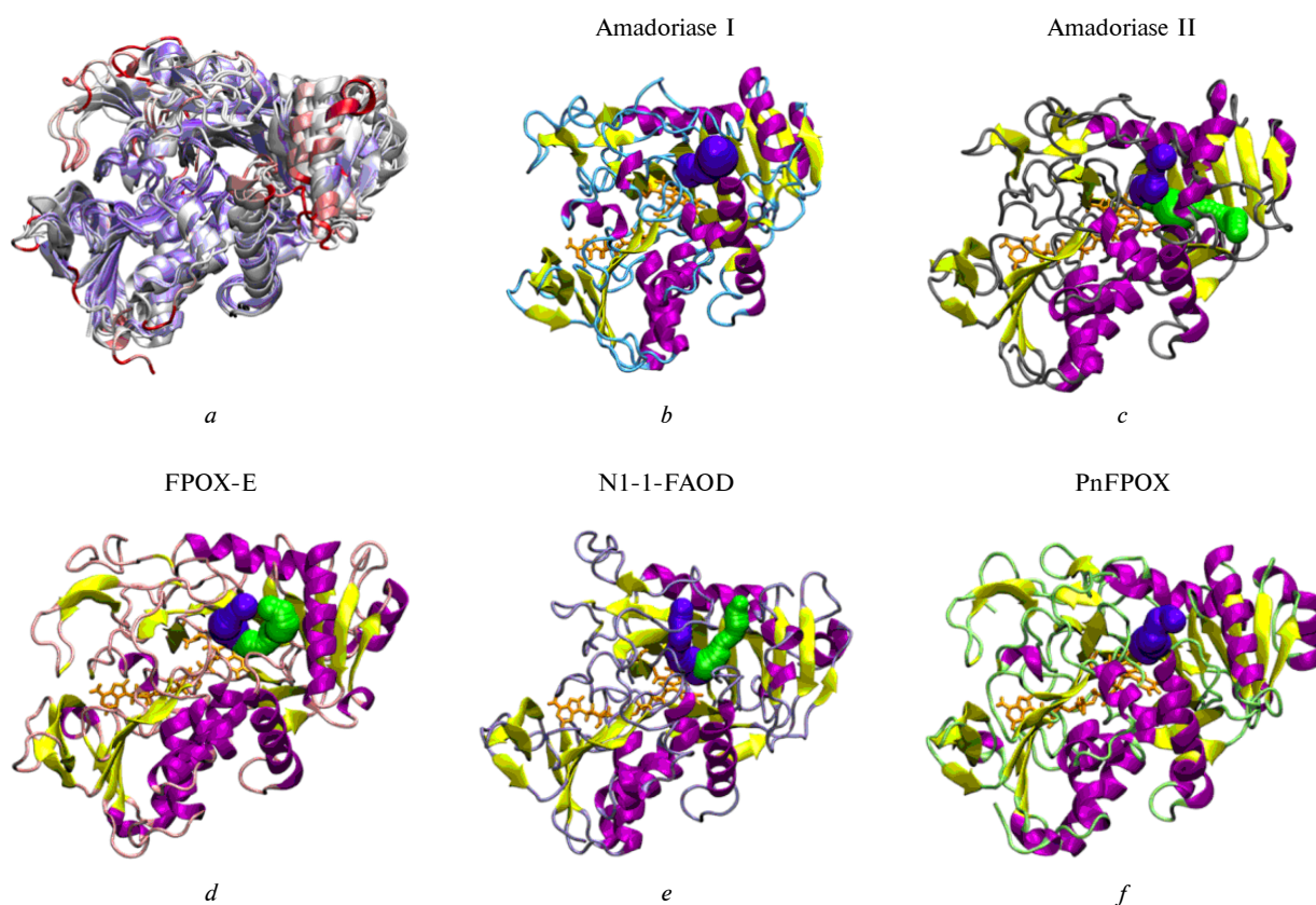
Fig. 3. FAOX structures. Superimposition of five wildtype enzyme structures colored by conserved regions ( a ). Blue, white and red indicate high, medium and low structure conservation regions, respectively. The remaining panels ( b-f ) show the overall folding and tunnel of the five FAOX. The main tunnel (shown in blue) is of similar length in all FAOX enzymes (14 Å)
