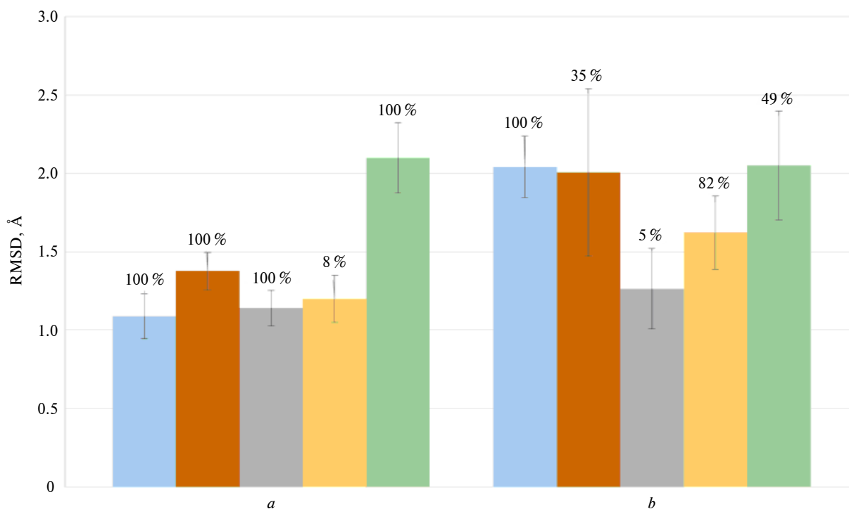
Fig. 4. Ligand stability. Root mean square deviation plots of the two ligands, measured over the time of the binding trajectory in which each ligand stays within the catalytic pocket (indicated above each bar): ■ – Amadoriase I; ■ – Amadoriase II; ■ – FPOX-E; ■ – N1-1-FAOD; ■ – PnFPOX; a – f-lys, b – f-val
