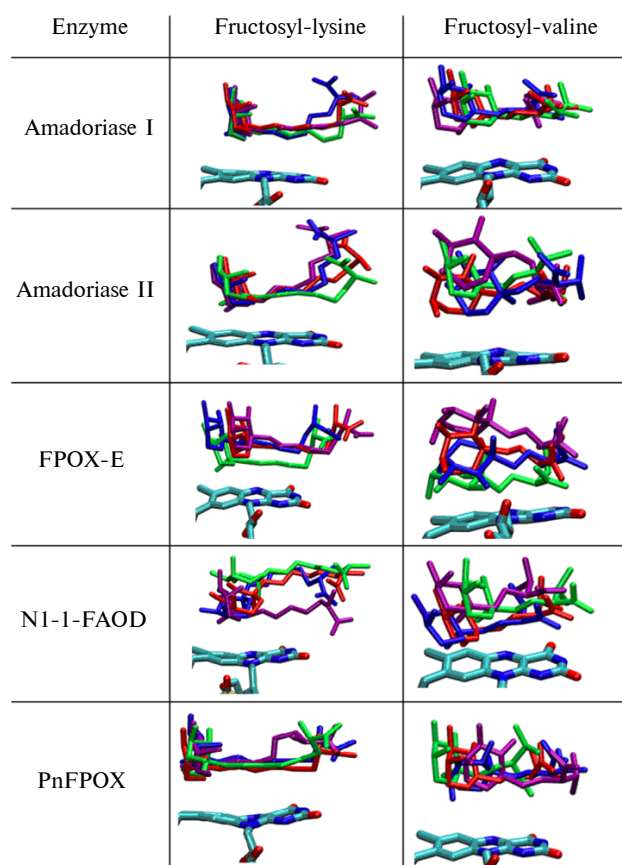
Fig. 5. Ligand conformational clusters. Each panel shows the four most common conformation clusters of f-lys and f-val inside the catalytic pocket of the five enzymes. The most populated cluster is shown in red, the second in blue and the others in green and purple, respectively. The flavin ring is shown for reference
