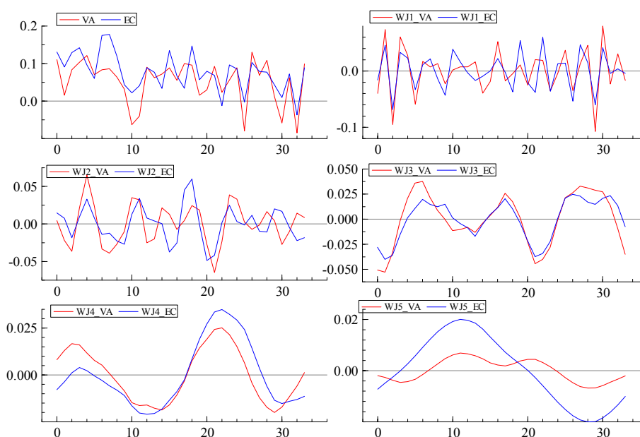
Fig. 1. MODWT wavelet coefficients of VA and EC
