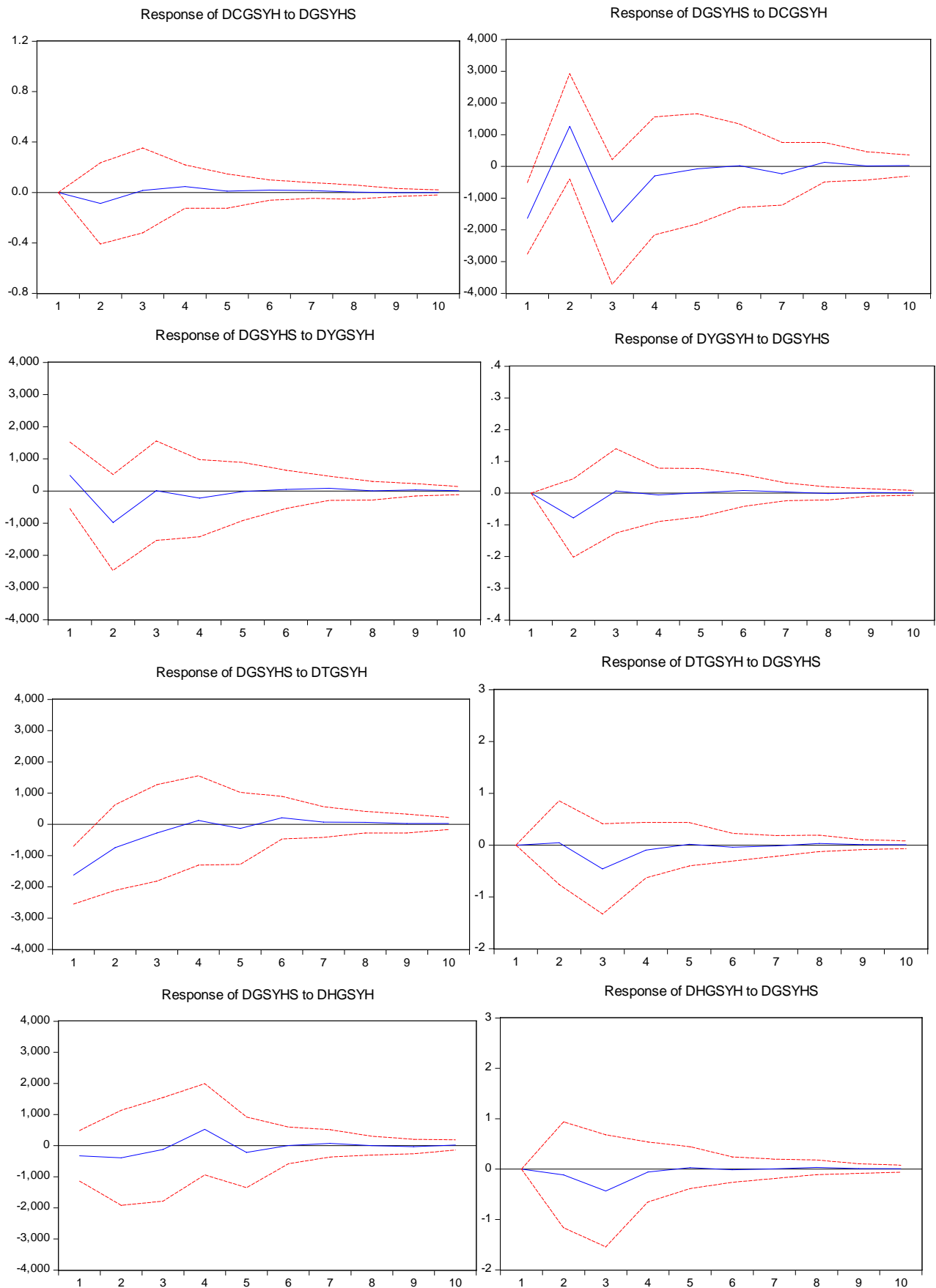
Fig. 1. Impulse-response functions
