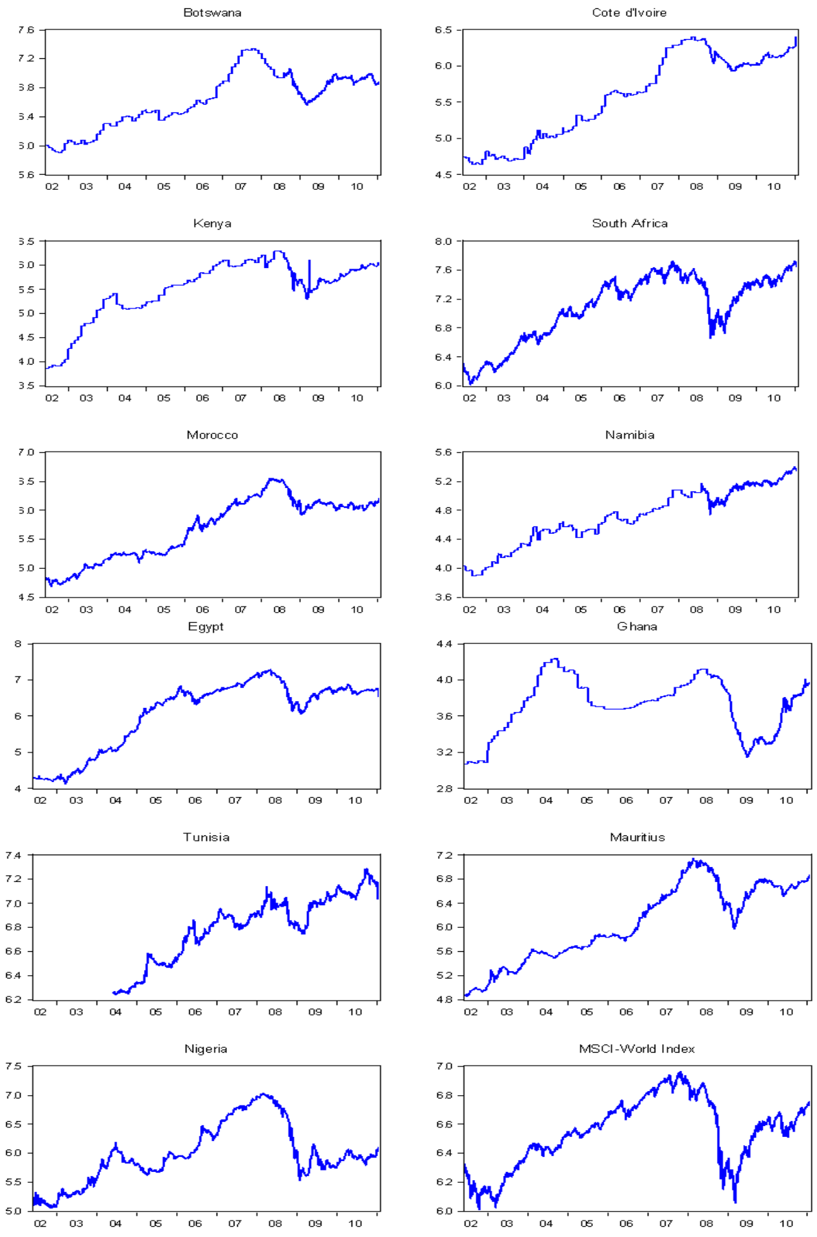
Fig. 1. Logarithms of daily stock prices
