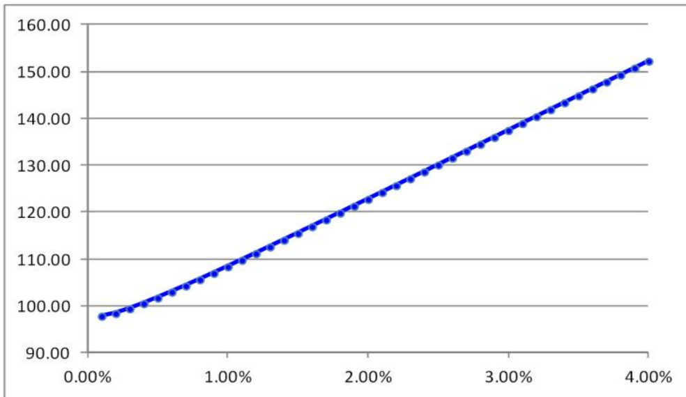
Fig. 3. Price sensitivity vs. F_t
