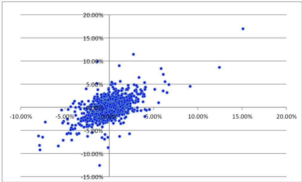
Fig. 1. Scatter plot of AT&T vs. MSFT returns
