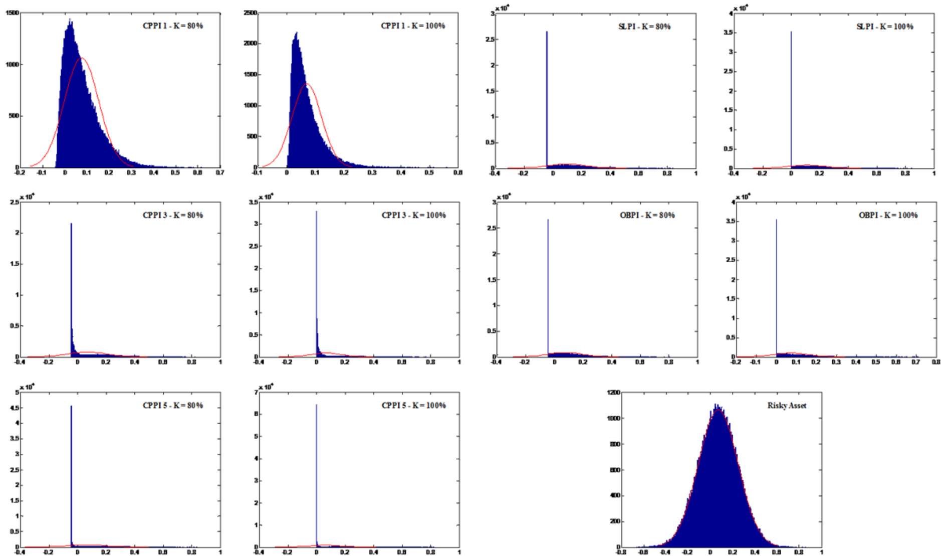
Notes: Probability density function of strategies returns – CPPI 1, CPPI 3, CPPI 5, SLPI, OBPI and Risky Asset. These results were achieved based on the following scenario: \mu = 15\% ; \sigma = 40\% ; r = 5\% ; T = 5 ; d = 252 ; N = 10.000 . For each strategy it was assumed a K = 80\% and a K = 100\% .
